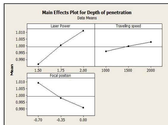
Figure 4 Main effects plot for DOP
