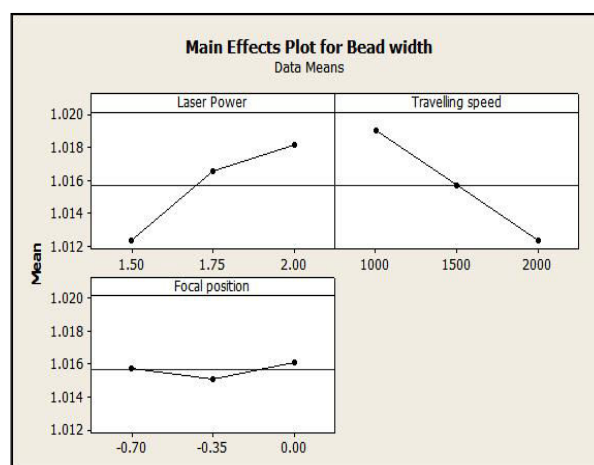
Figure 5 Main effects plot for bead width
